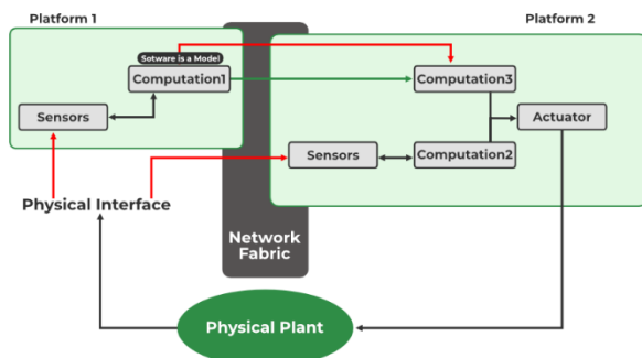
Fig. 2. Next-generation cyber-physical network plant.
